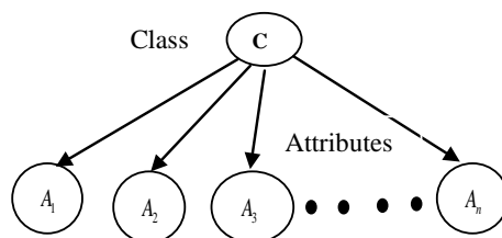
Figure 1. Structure of a naïve Bayes network.
